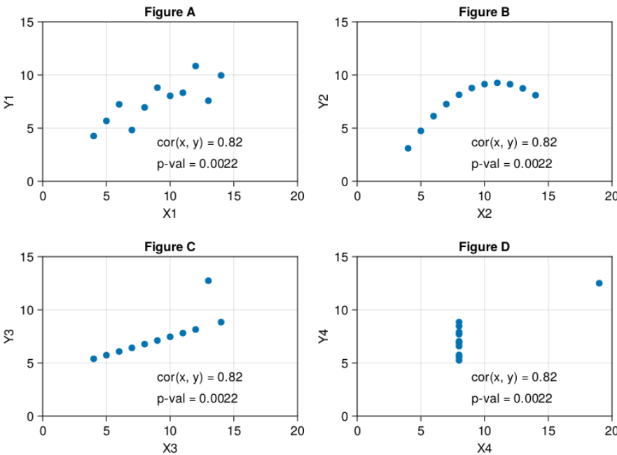
Figure 7.3: Anscombe's Quartet.
